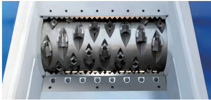
动刀采用DC53合金，定刀采用D2合金。 Rotary knife adopts DC53 steel, counter knife adopts D2. 动刀可角使用后再更换。 Rotary knife can be used twice before replaced.
